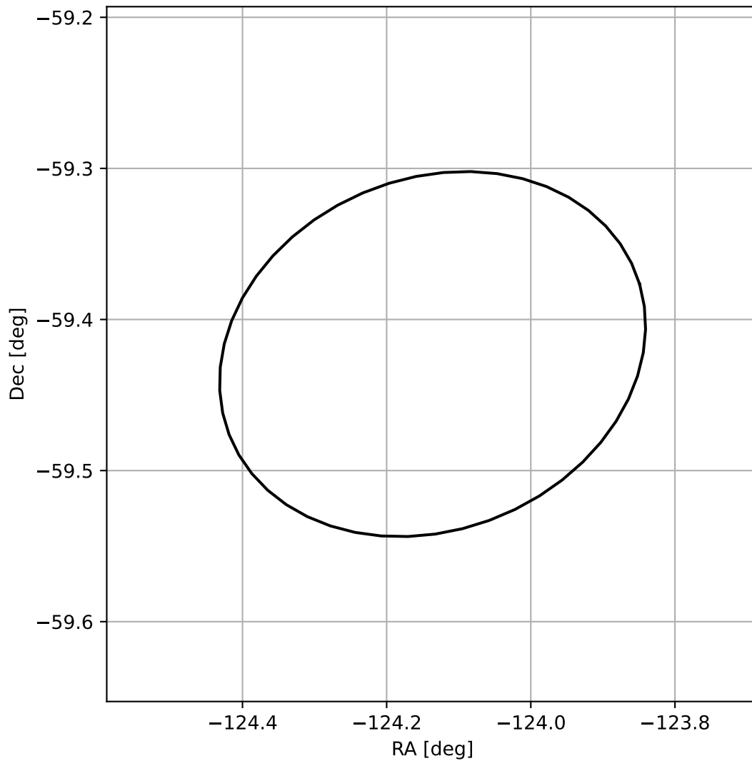
4FGL J1543.4-5925
