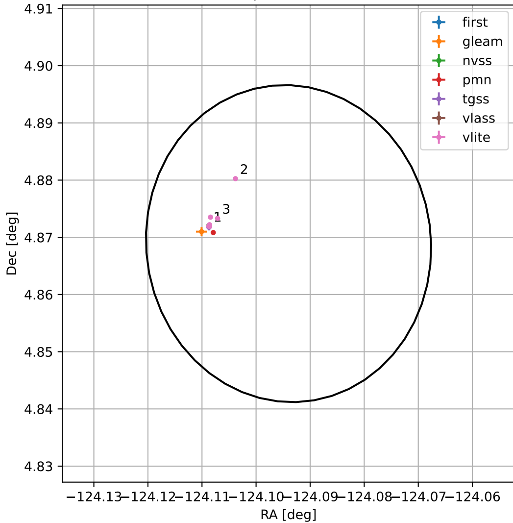
4FGL J1543.6+0452
