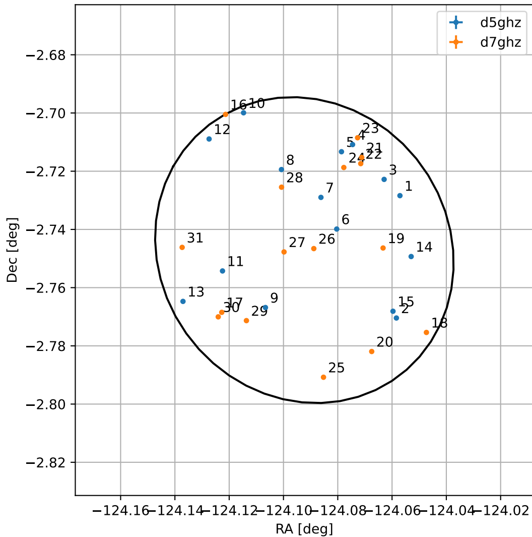
4FGL J1543.6-0244
