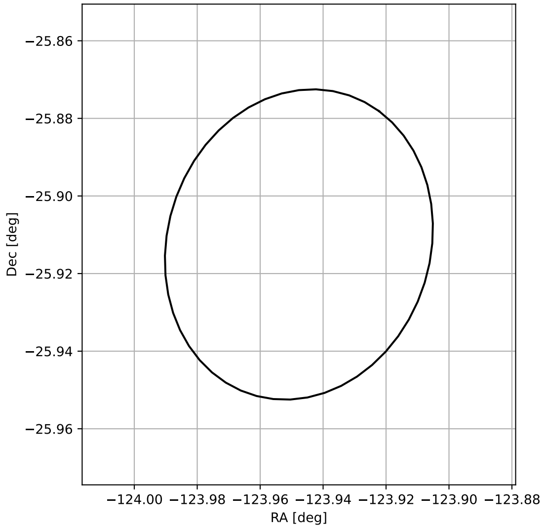
4FGL J1544.2-2554
