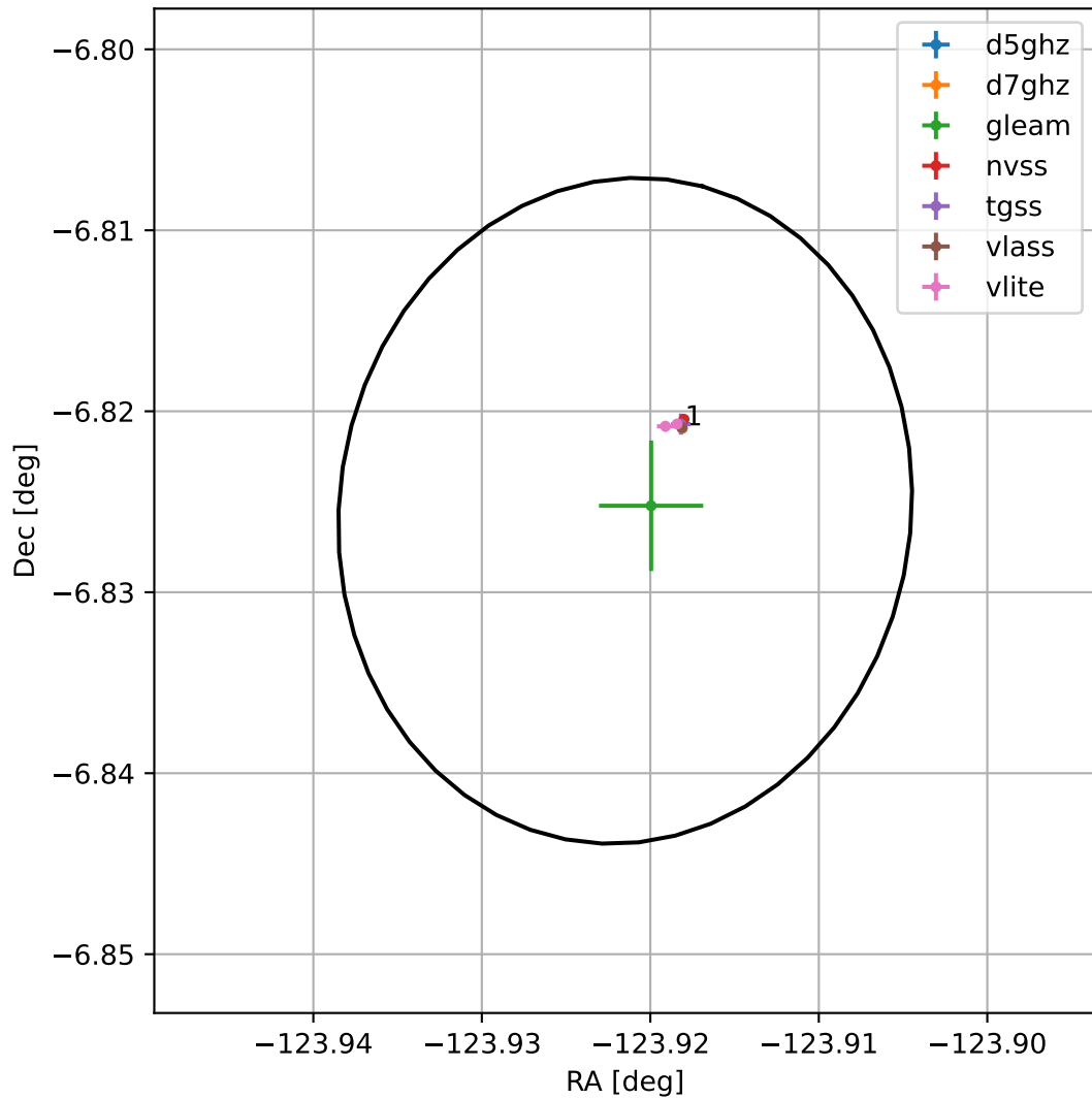
4FGL J1544.3-0649
