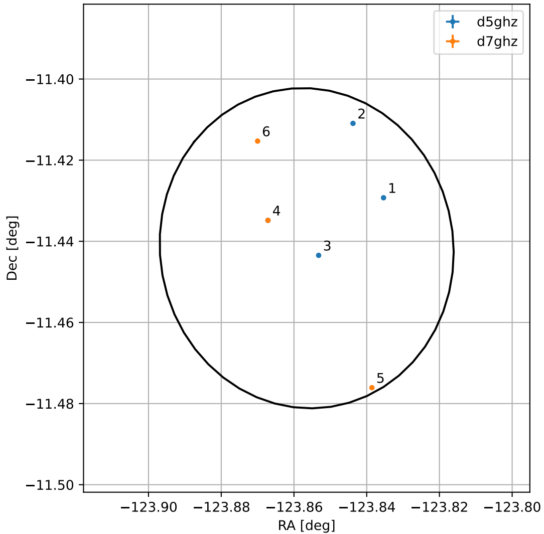
4FGL J1544.5-1126
