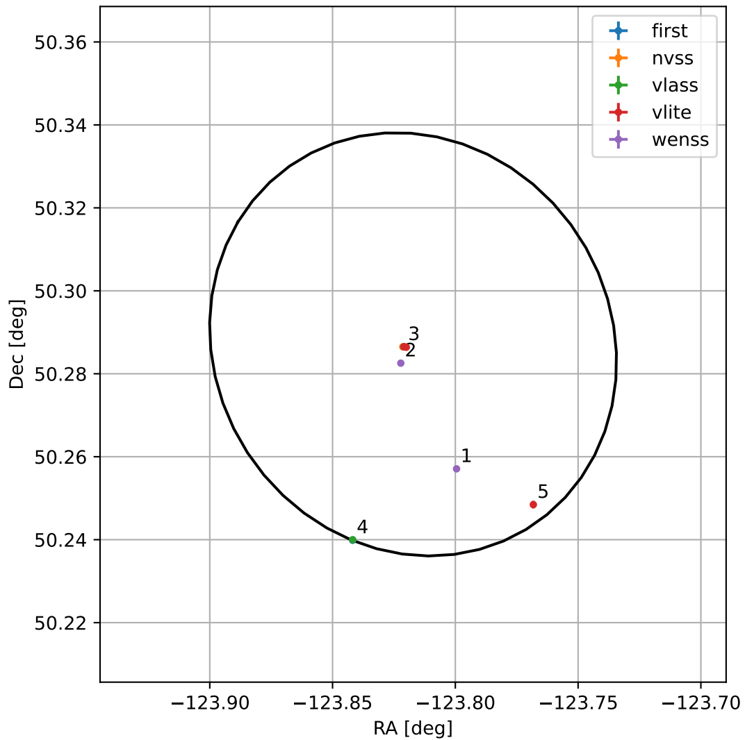
4FGL J1544.7+5017
