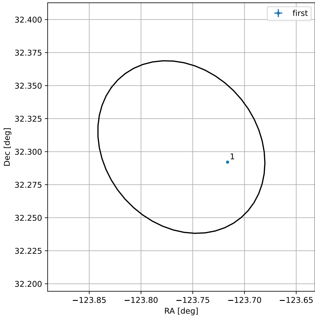
4FGL J1544.9+3218
