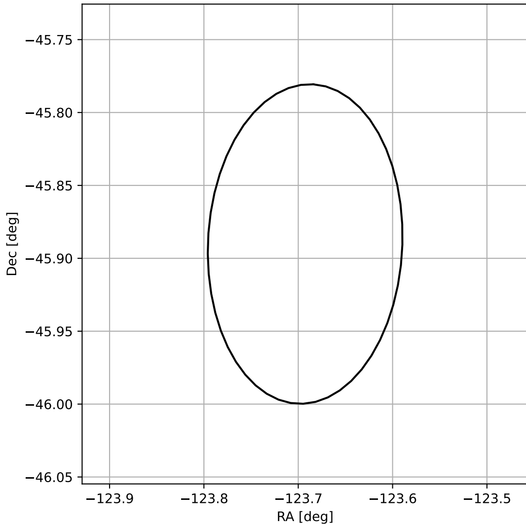
4FGL J1545.2-4553
