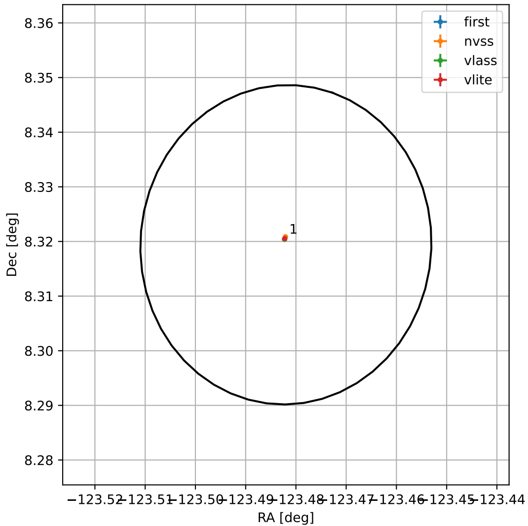
4FGL J1546.0+0819
