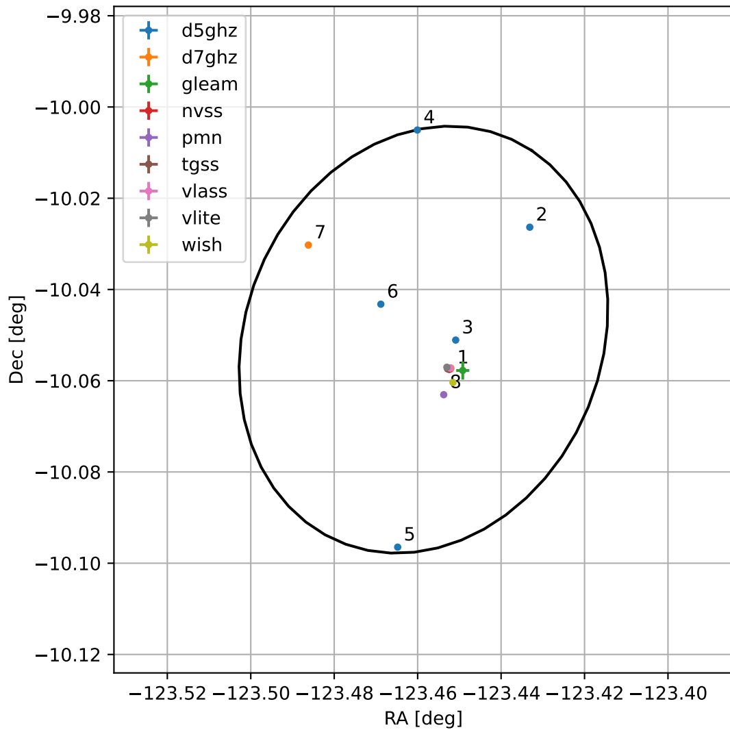
4FGL J1546.1-1003
