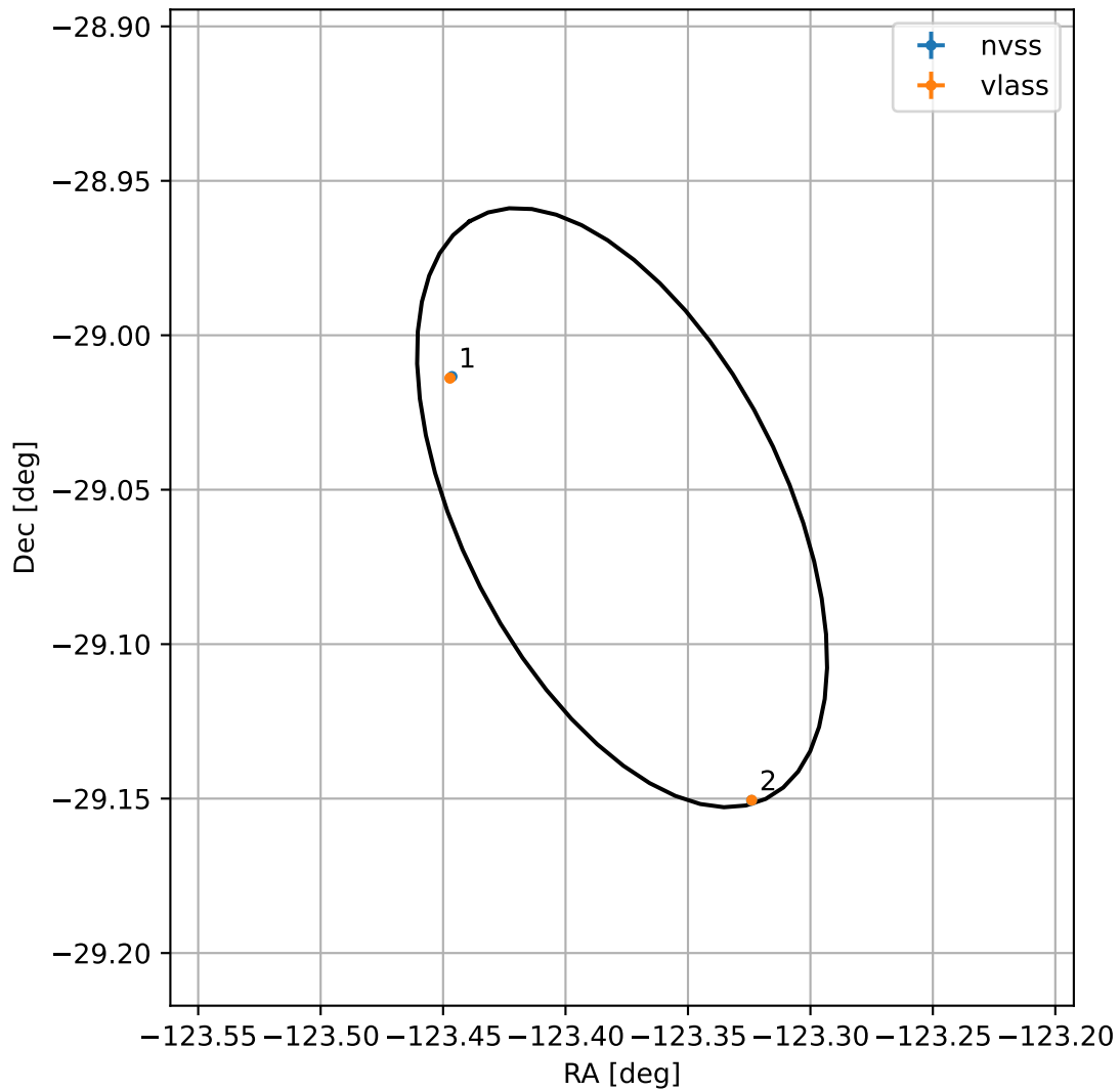
4FGL J1546.4-2903
