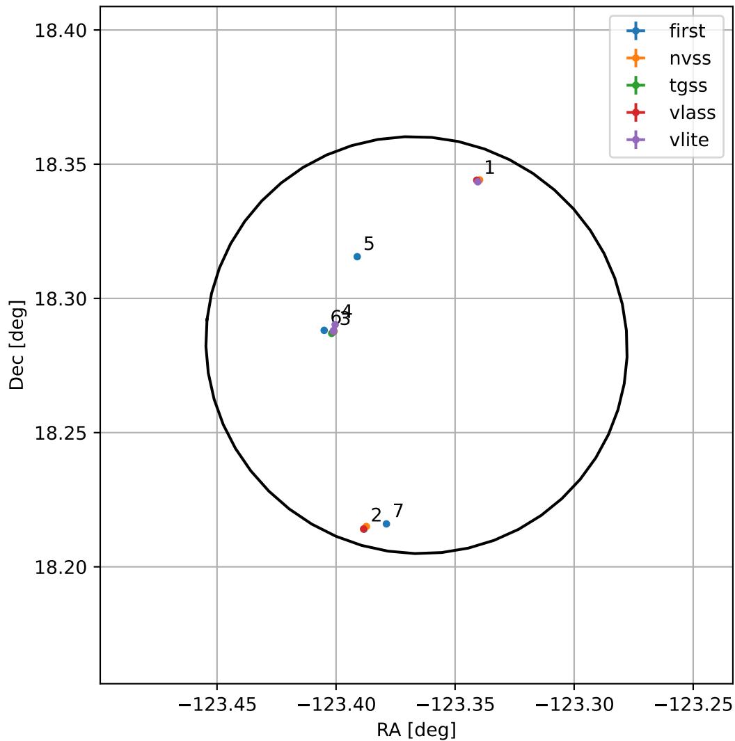
4FGL J1546.5+1816
