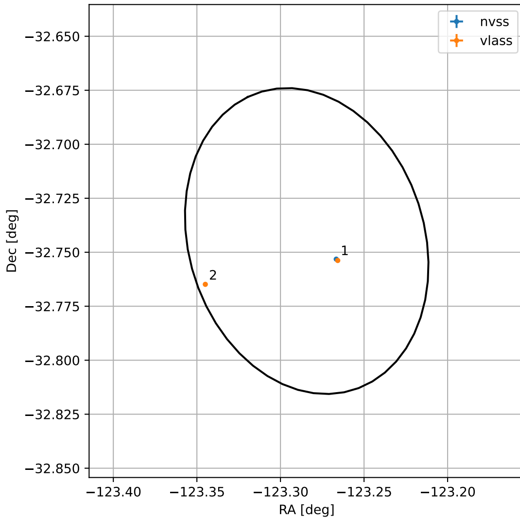
4FGL J1546.8-3244
