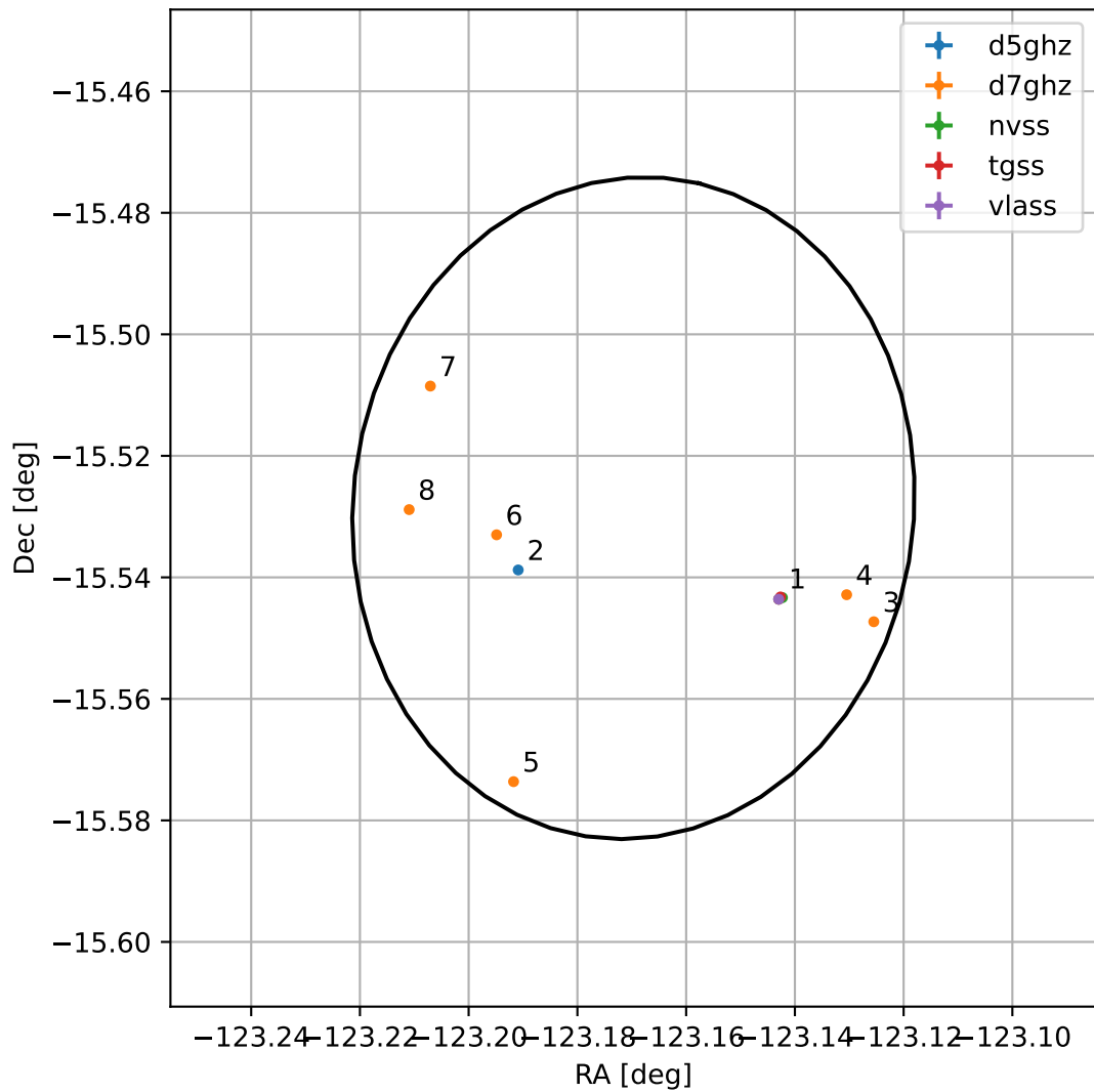
4FGL J1547.3-1531
