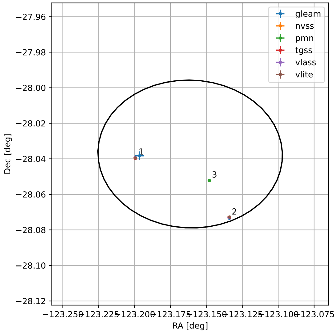
4FGL J1547.3-2802
