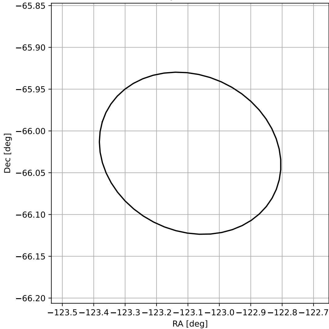
4FGL J1547.6-6601
