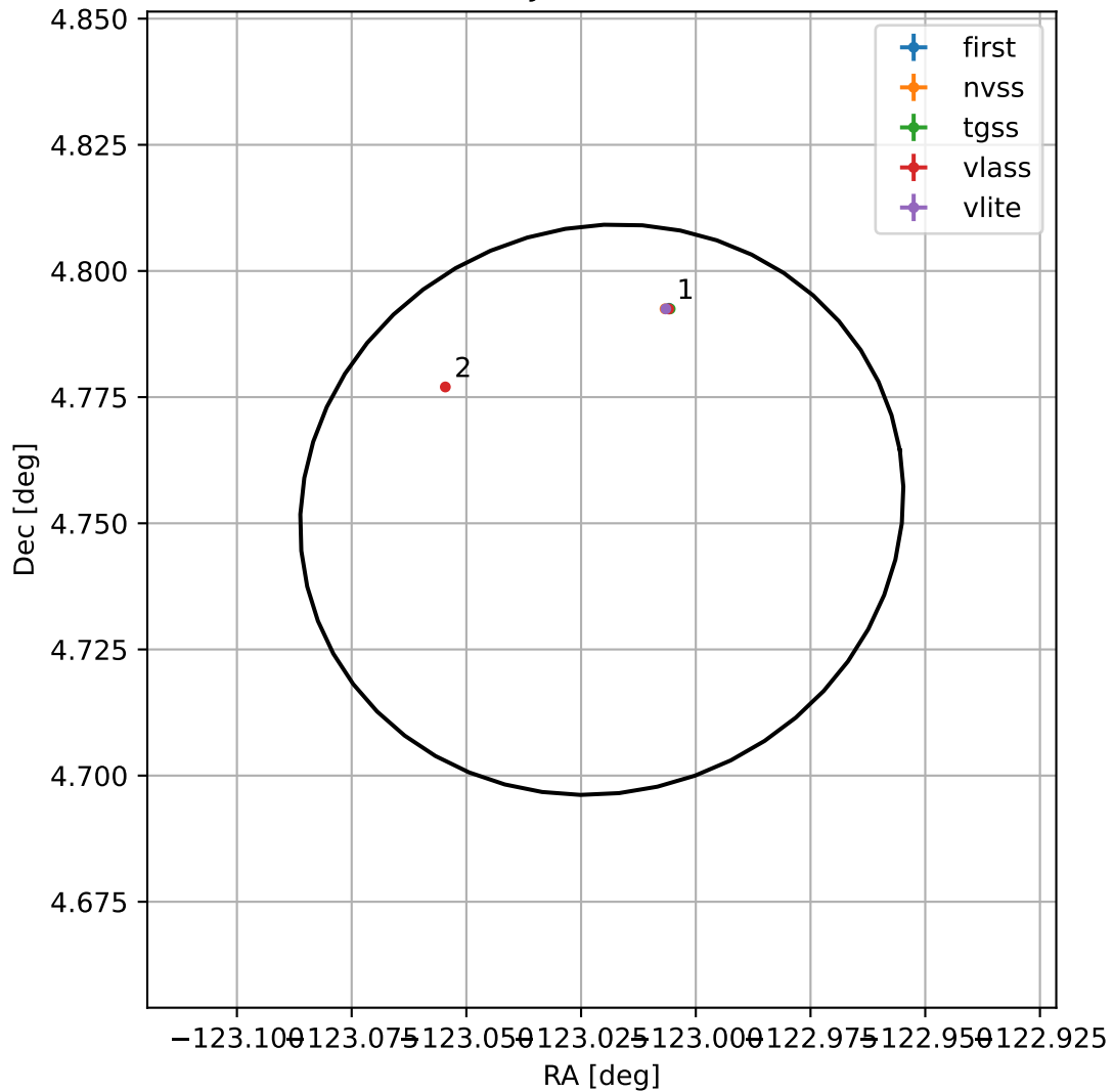
4FGL J1547.9+0445
