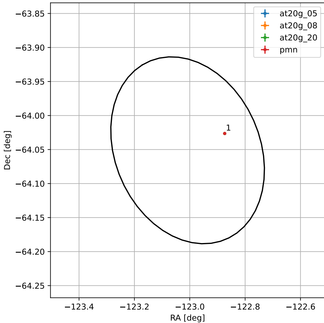
4FGL J1547.9-6403
