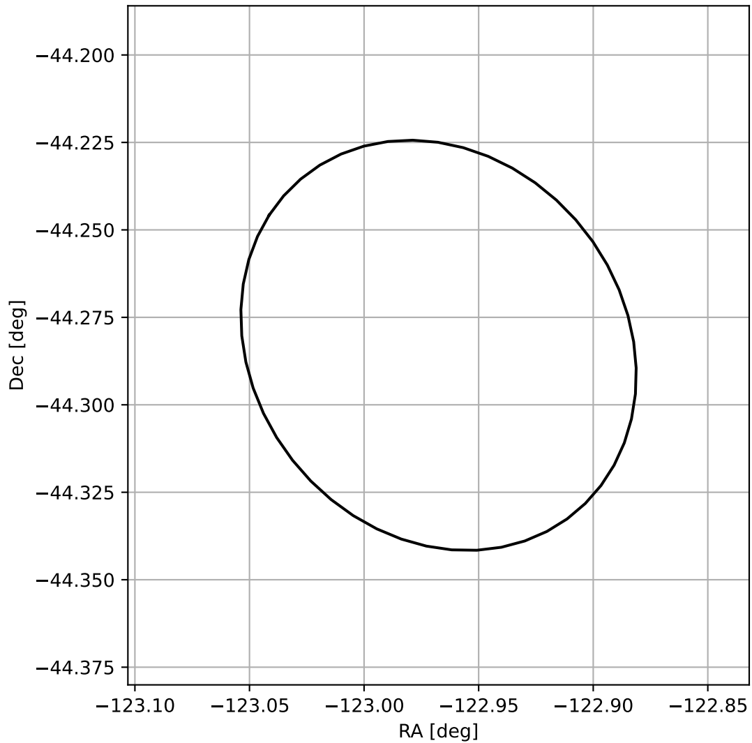
4FGL J1548.1-4416
