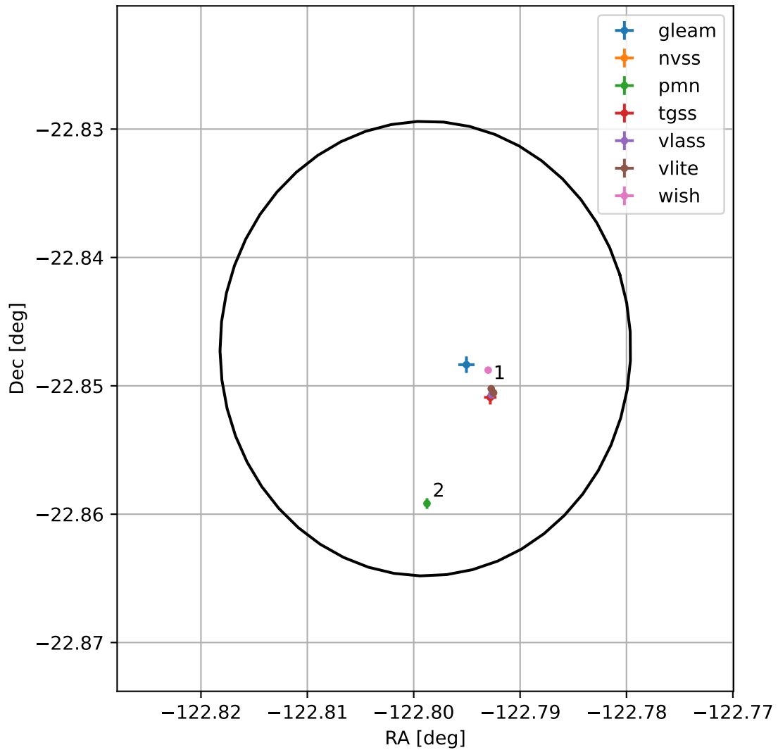
4FGL J1548.8-2250
