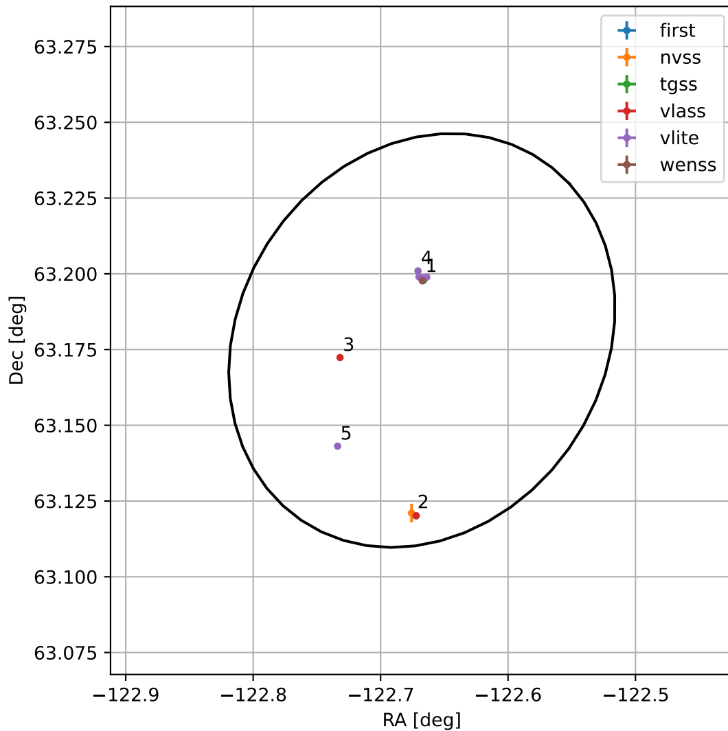
4FGL J1549.3+6310
