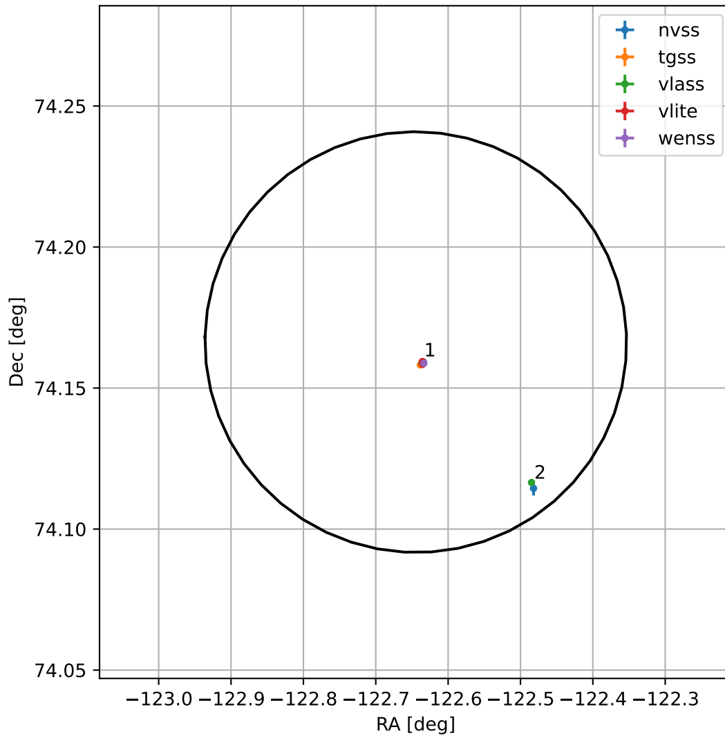
4FGL J1549.4+7409
