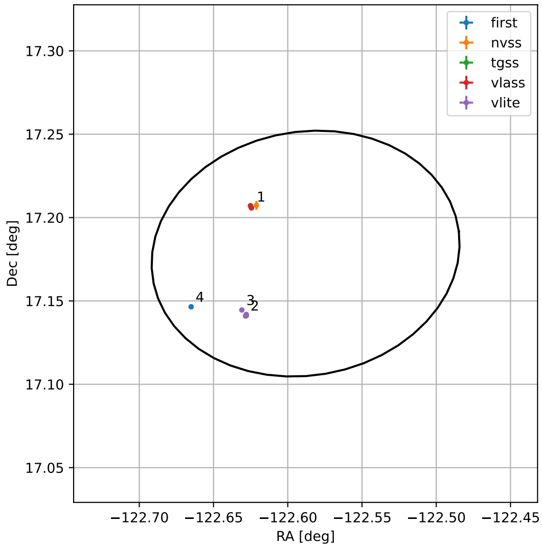
4FGL J1549.6+1710
