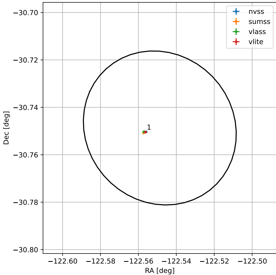
4FGL J1549.8-3044
