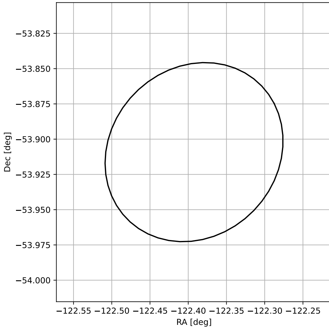
4FGL J1550.4-5354
