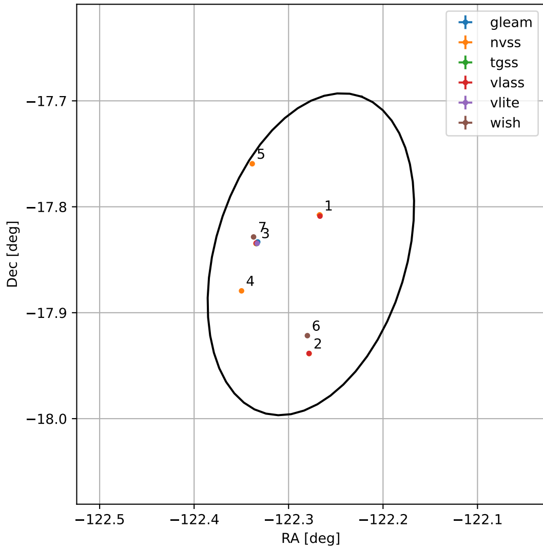
4FGL J1550.8-1750
