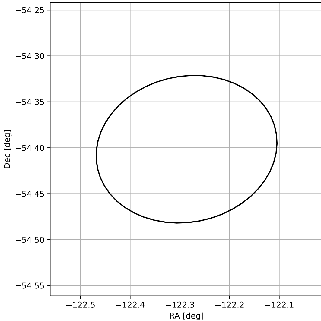
4FGL J1550.8-5424
