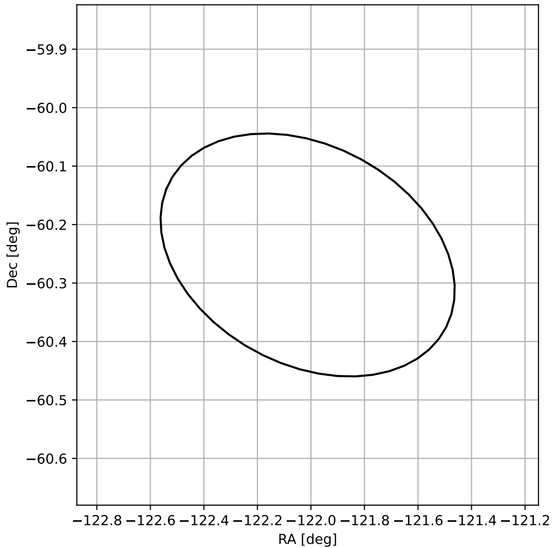
4FGL J1551.9-6015
