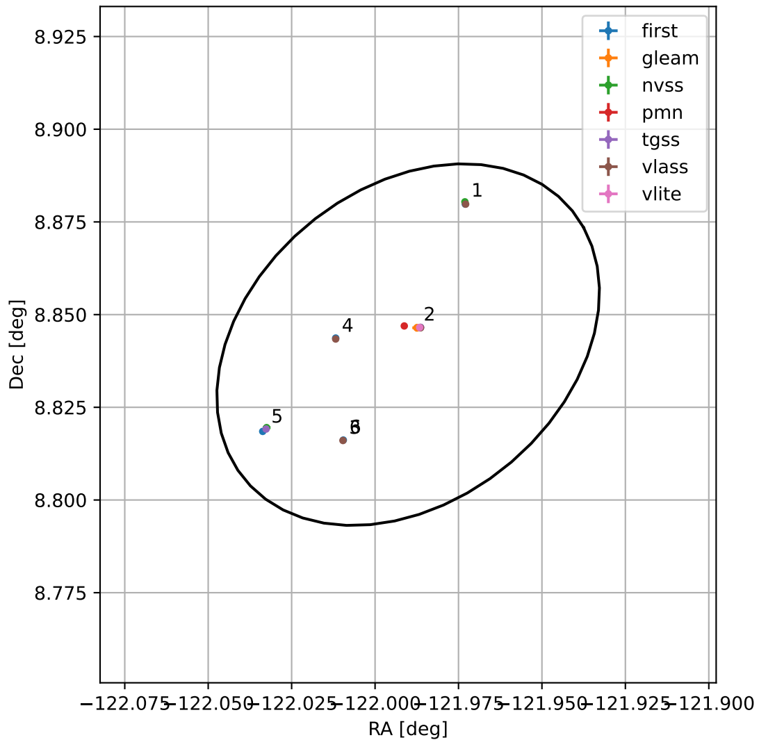
4FGL J1552.0+0850
