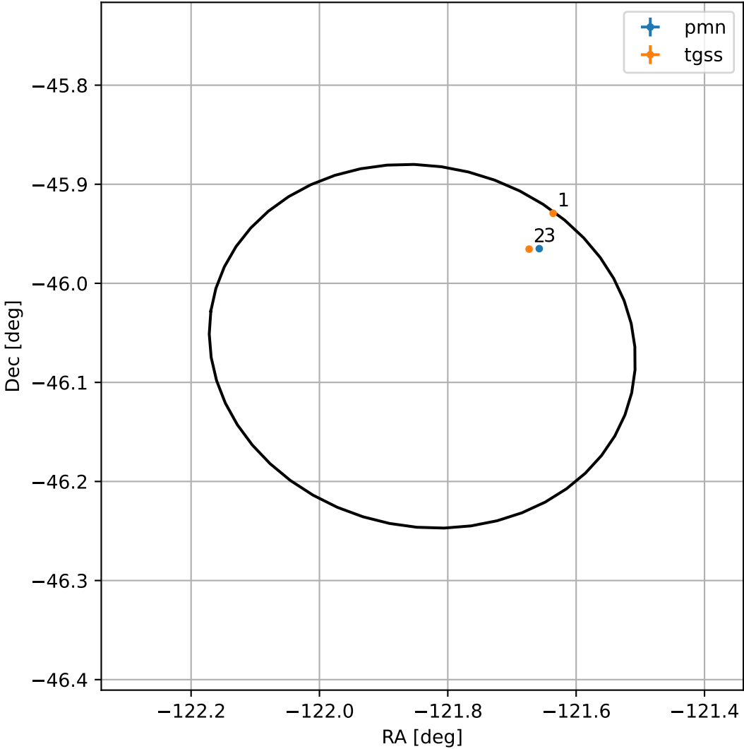
4FGL J1552.6-4603
