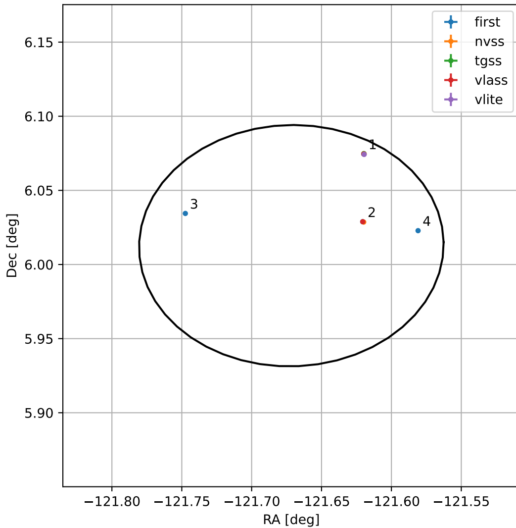
4FGL J1553.3+0600
