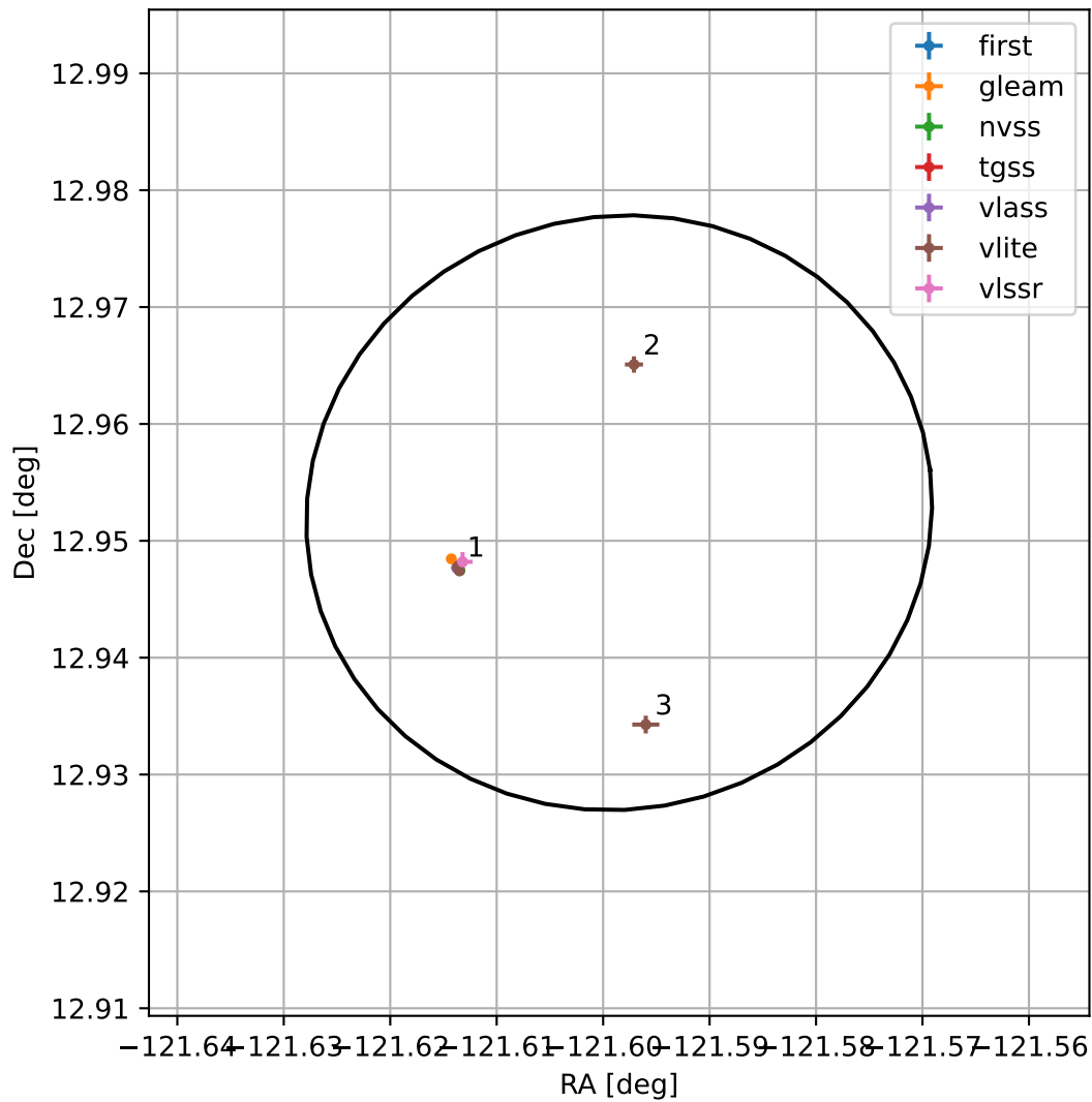
4FGL J1553.6+1257
