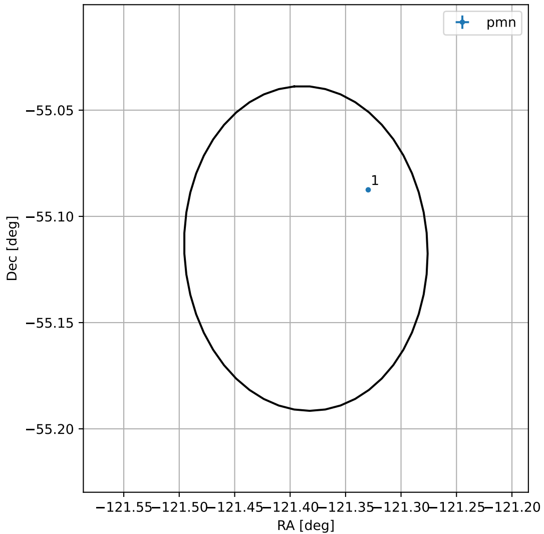
4FGL J1554.4-5506
