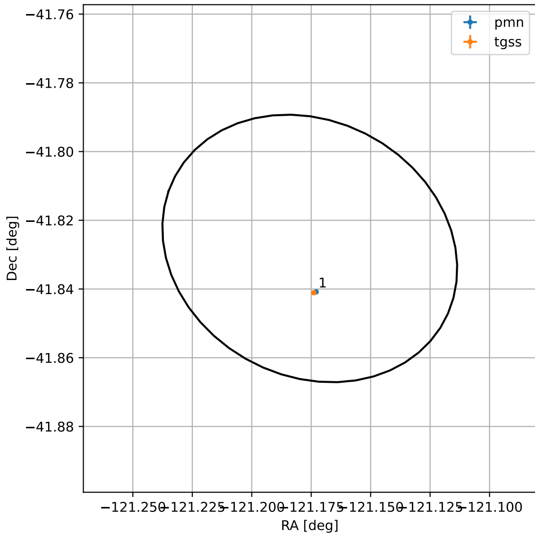
4FGL J1555.2-4149
