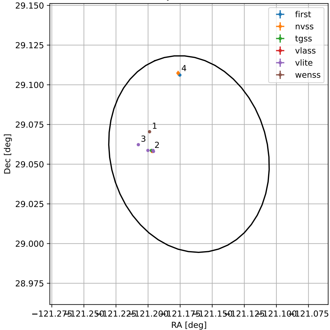
4FGL J1555.3+2903
