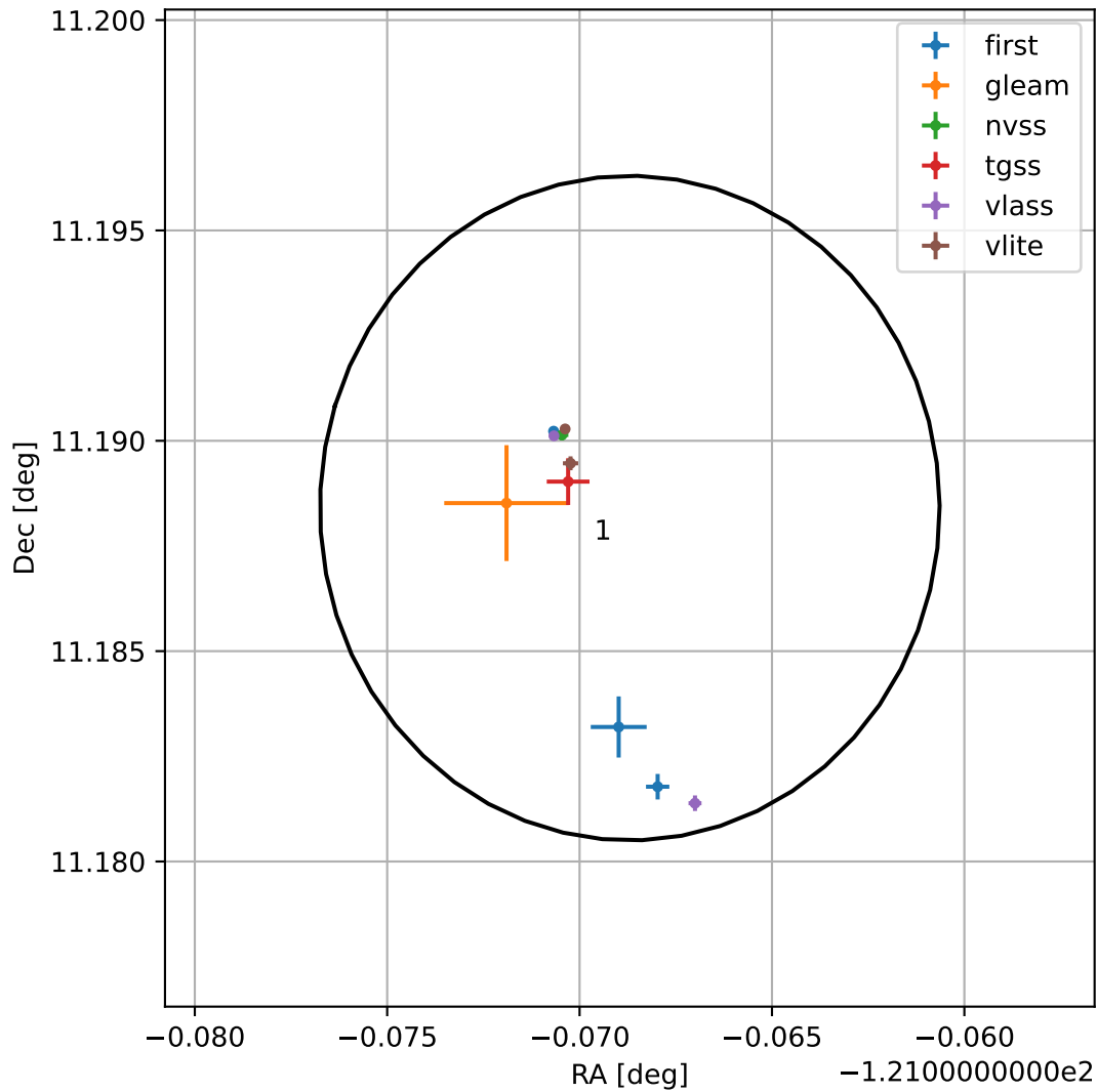
4FGL J1555.7+1111
