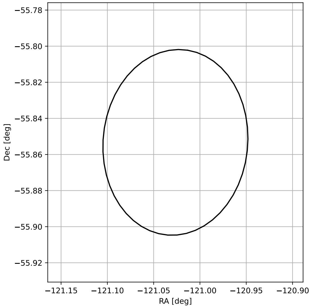
4FGL J1555.8-5551
