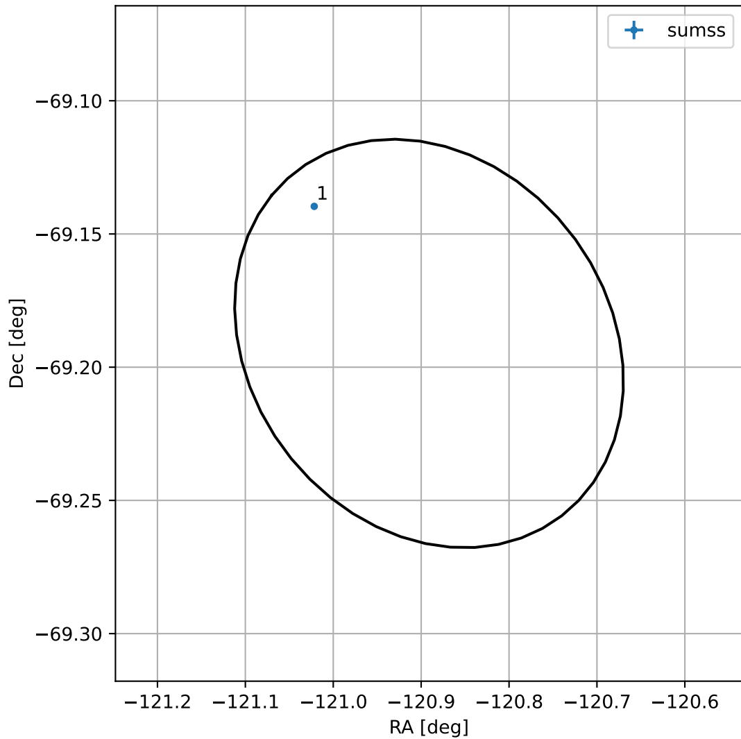
4FGL J1556.4-6911
