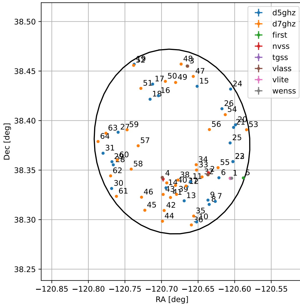
4FGL J1557.2+3822
