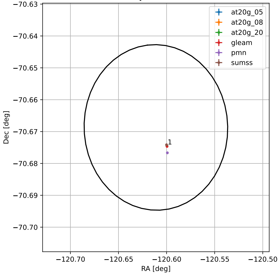
4FGL J1557.5-7040
