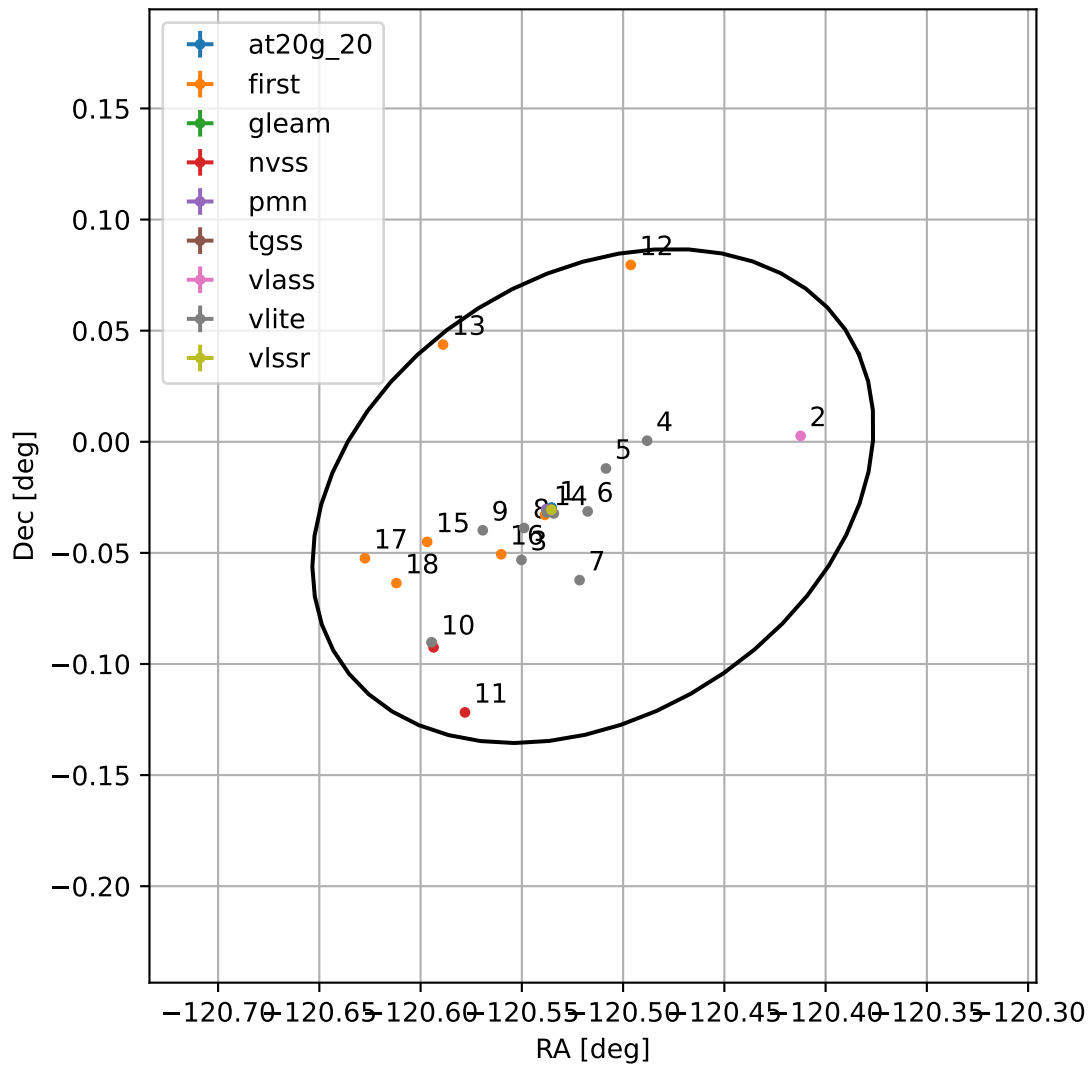
4FGL J1557.9-0001
