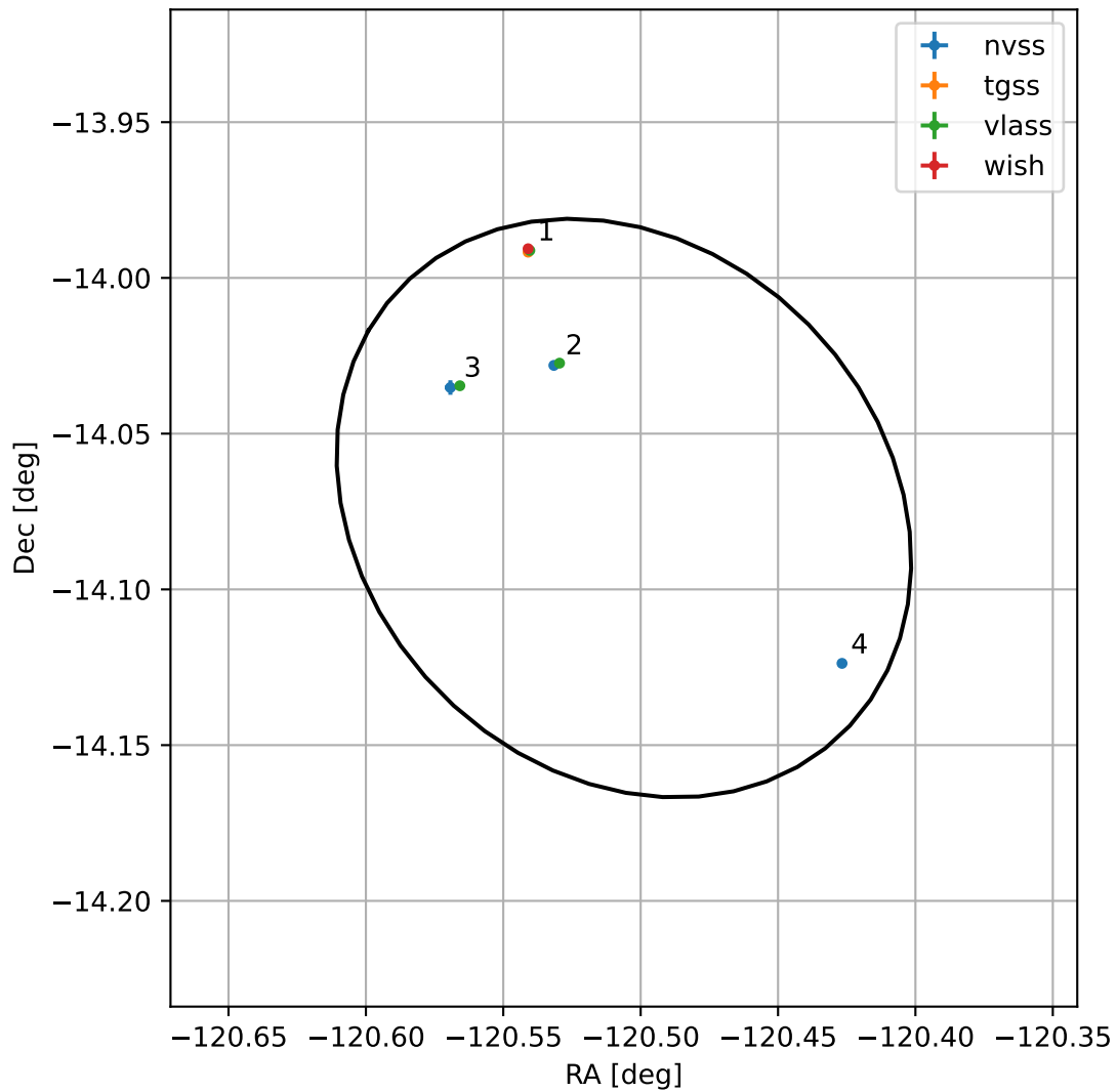
4FGL J1557.9-1404
