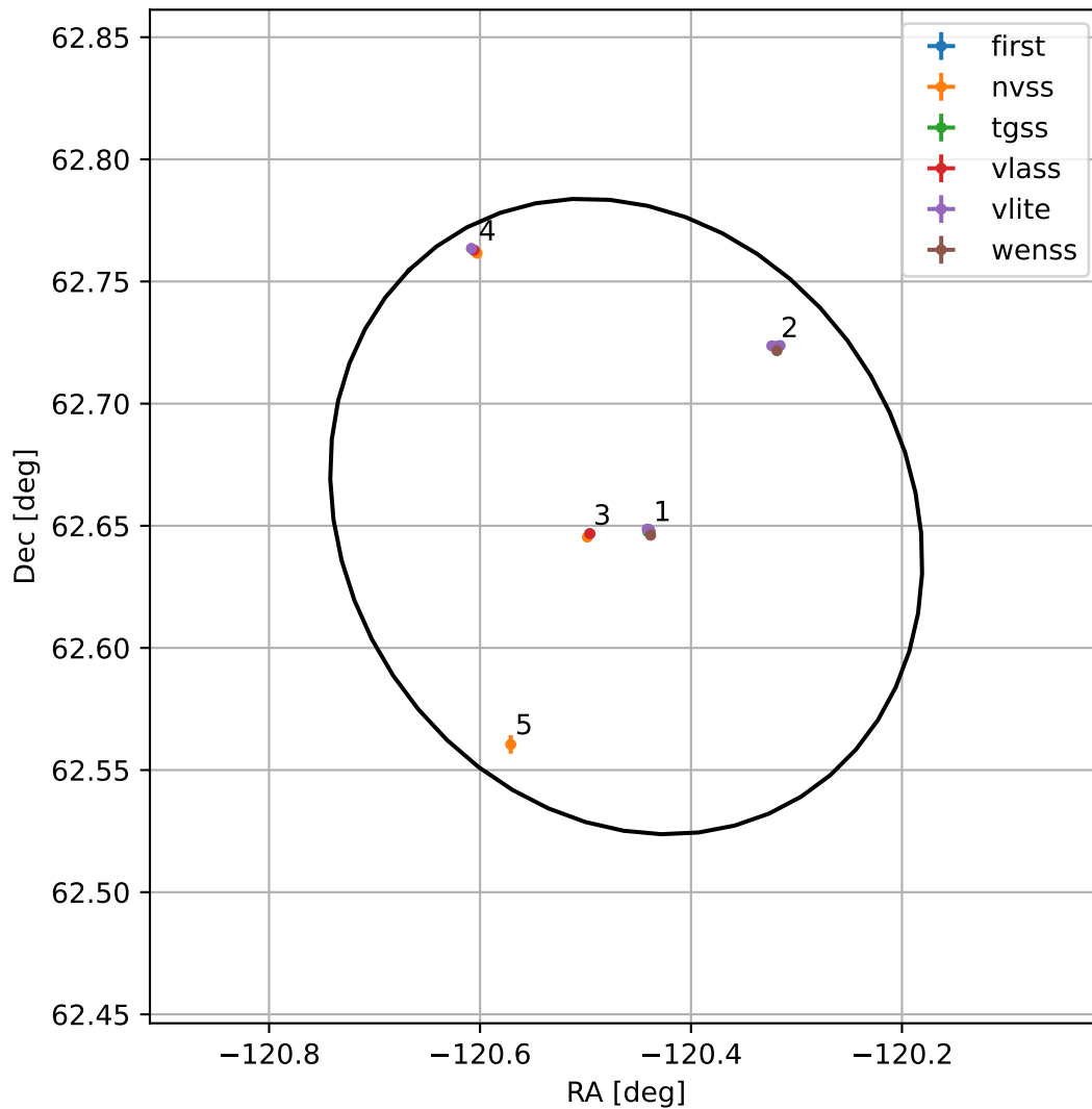
4FGL J1558.1+6239
