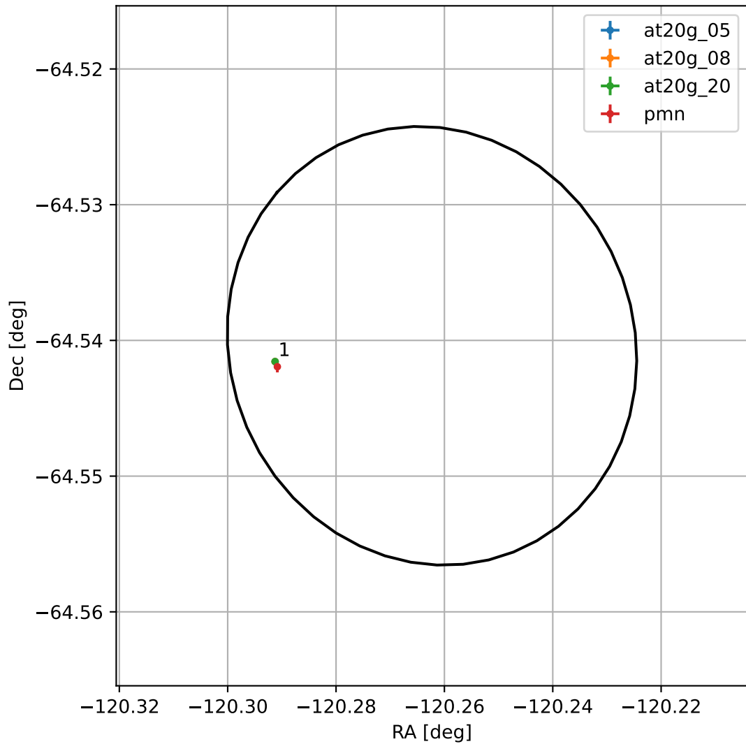
4FGL J1558.9-6432
