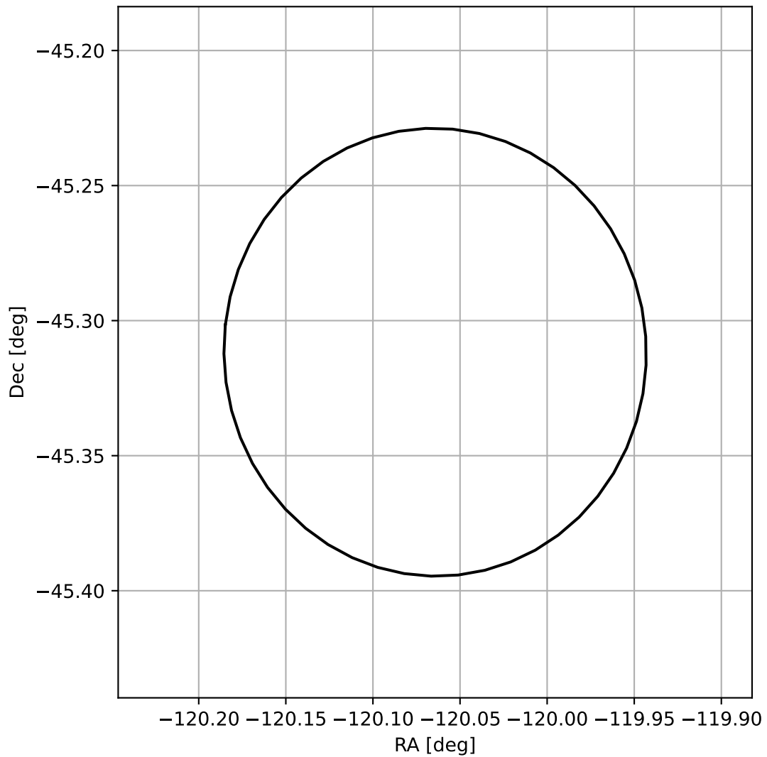
4FGL J1559.7-4518
