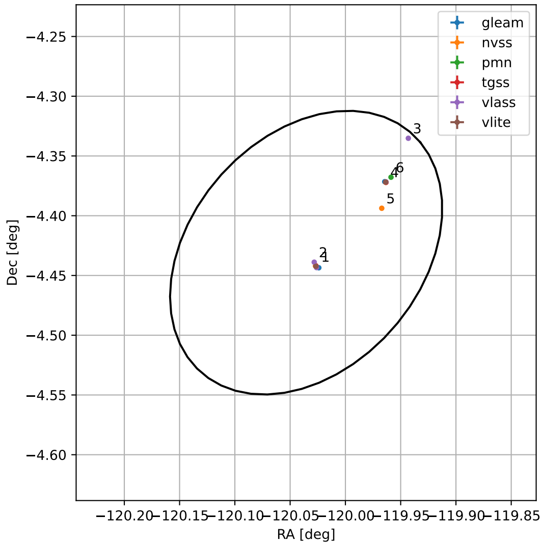
4FGL J1559.8-0425
