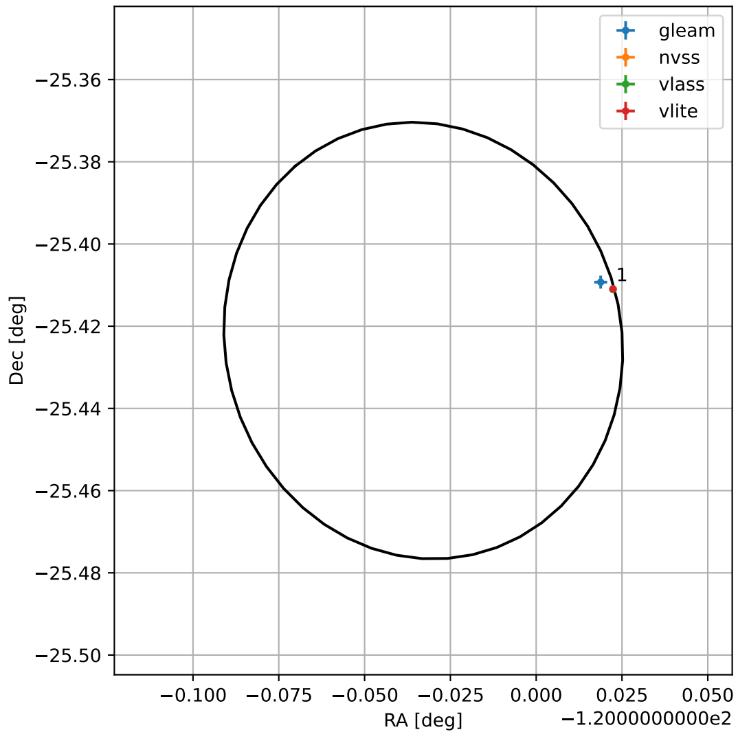
4FGL J1559.8-2525
