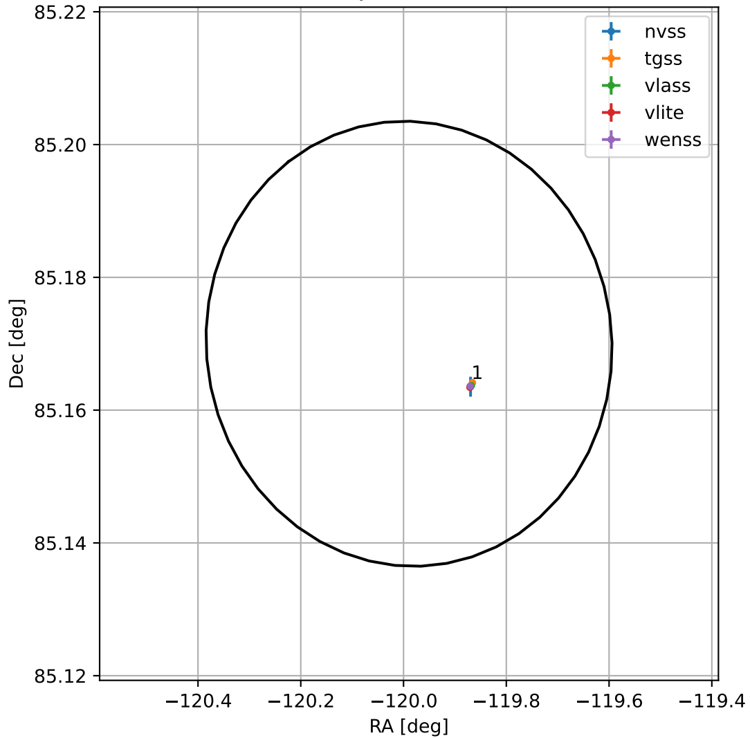
4FGL J1600.0+8510
