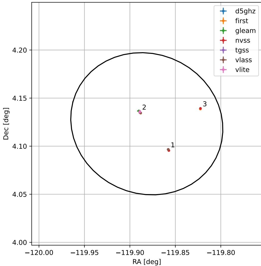
4FGL J1600.4+0407
